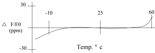
温度曲线图 Temperature Curve
