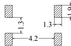
建议电路板印刷底座 Recommended Solder Pad Layout
