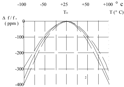
频率温度曲线图 Frequency Temperature Curve
